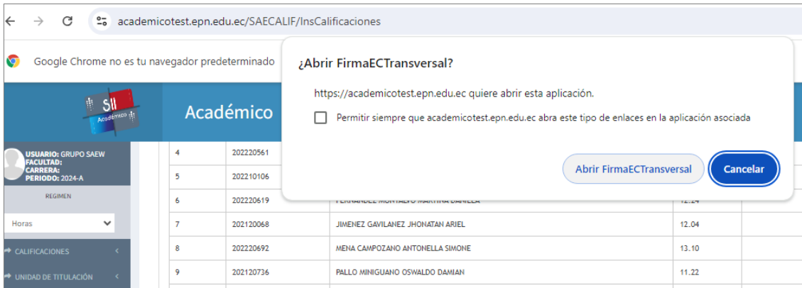
Figura 11: Abrir FirmaEC.
